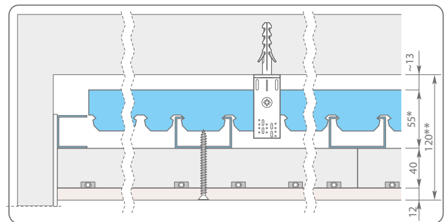
Structure with snap profile
