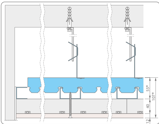
Hanging structure with snap profile
